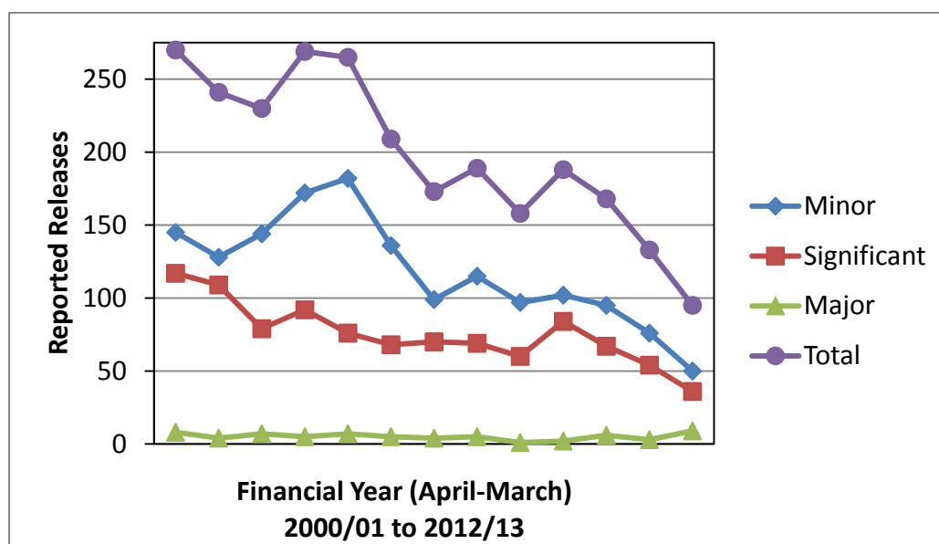
Figure 3. Hydrocarbon releases in the North Sea reported to UK HSE as dangerous occurrences under the Reporting of Injuries, Diseases and Dangerous Occurrences Regulations. 476
